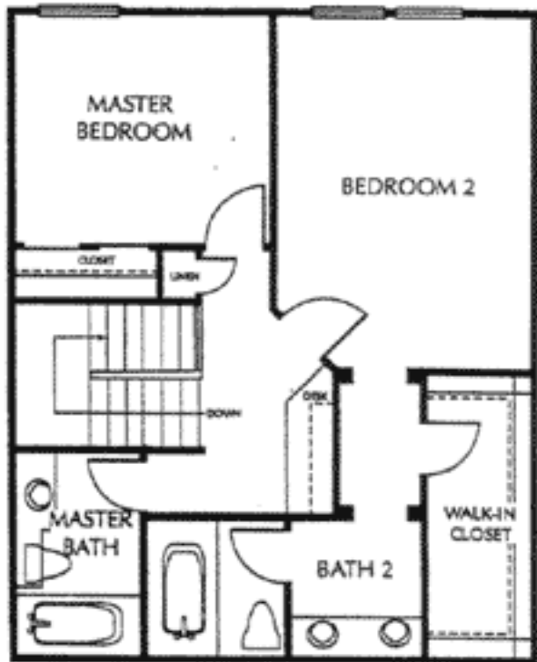
SECOND STORY
